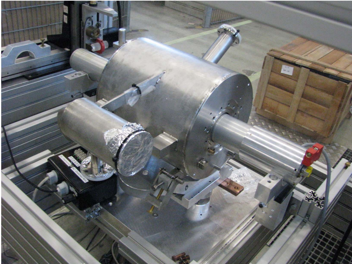
Cold magnet in its helium vessel on a test stand
