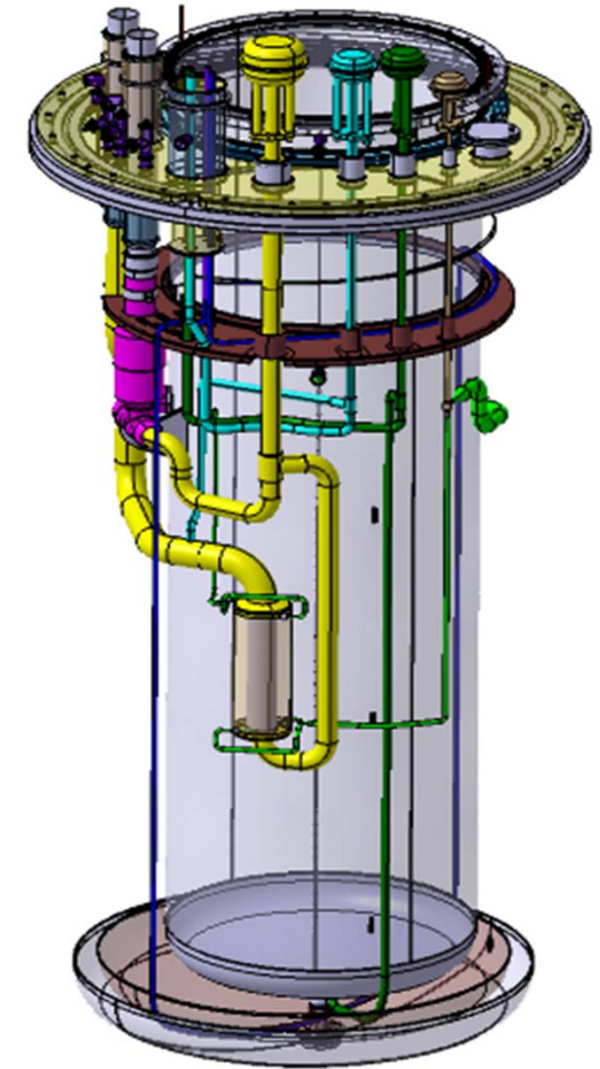
Cryostat for testing superconducting cavities
