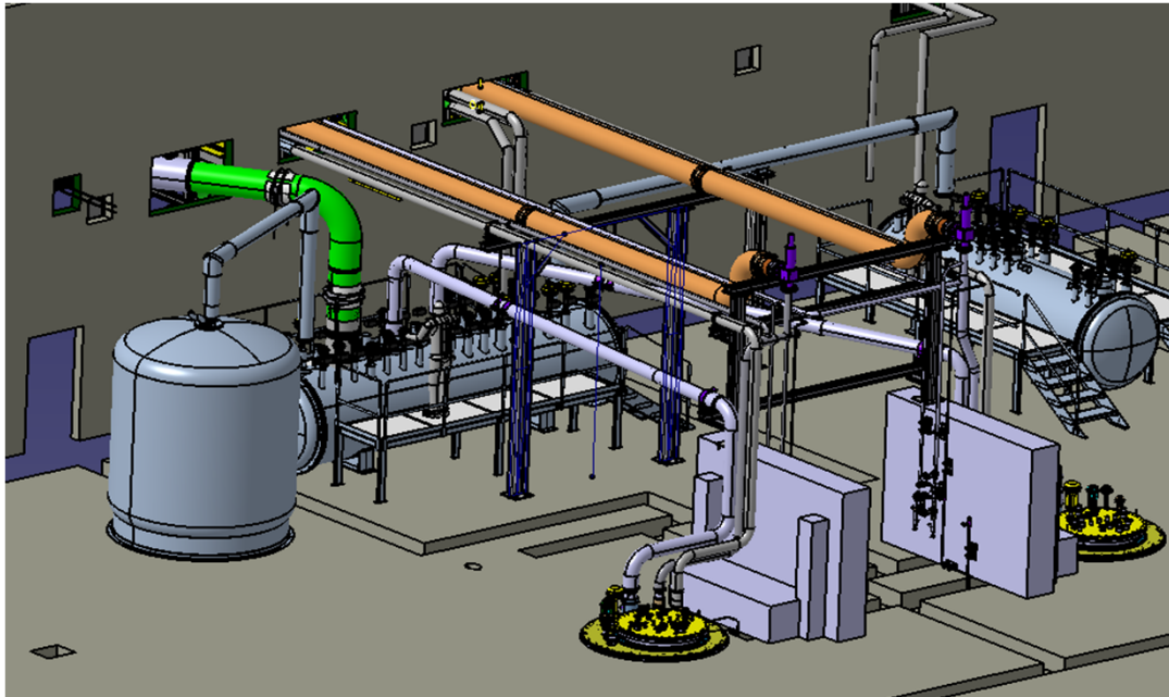
Layout of cryogenic system for the cavities tests in AMTF hall
